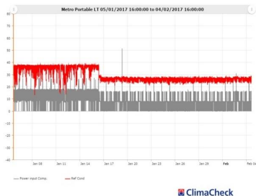
Figure 5, Power before and after measures
