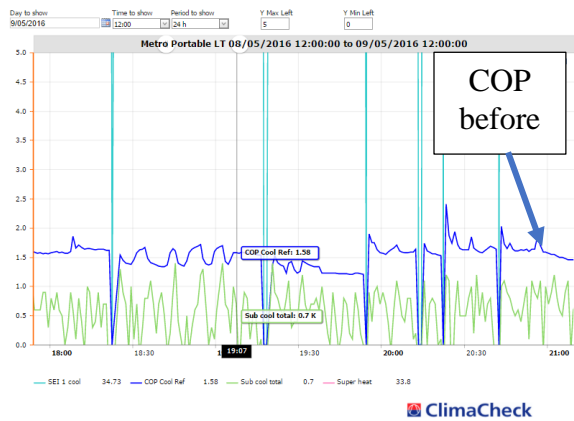
Figure 4, COP before and after measures
