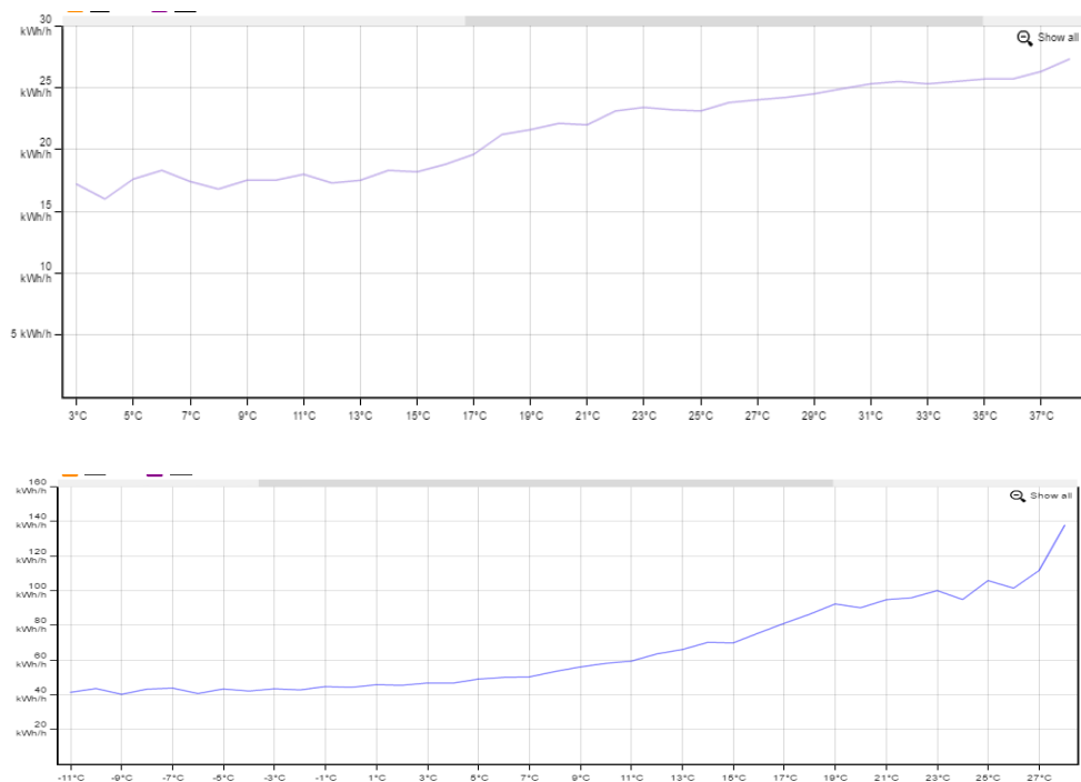
Figure 2, Typical energy signature Greece and Sweden
