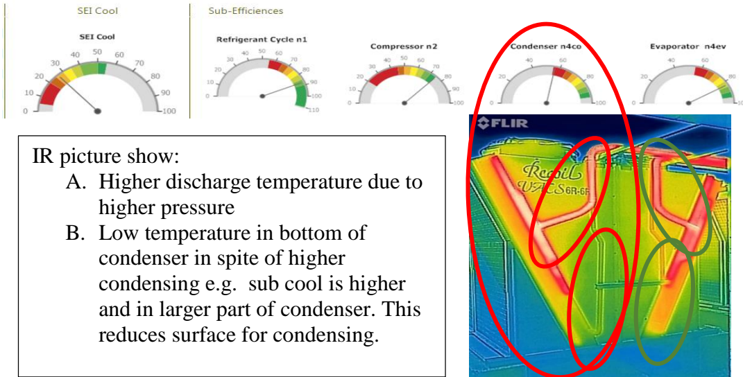
Figure 7, Air-cooled chiller with too much refrigerant charge
