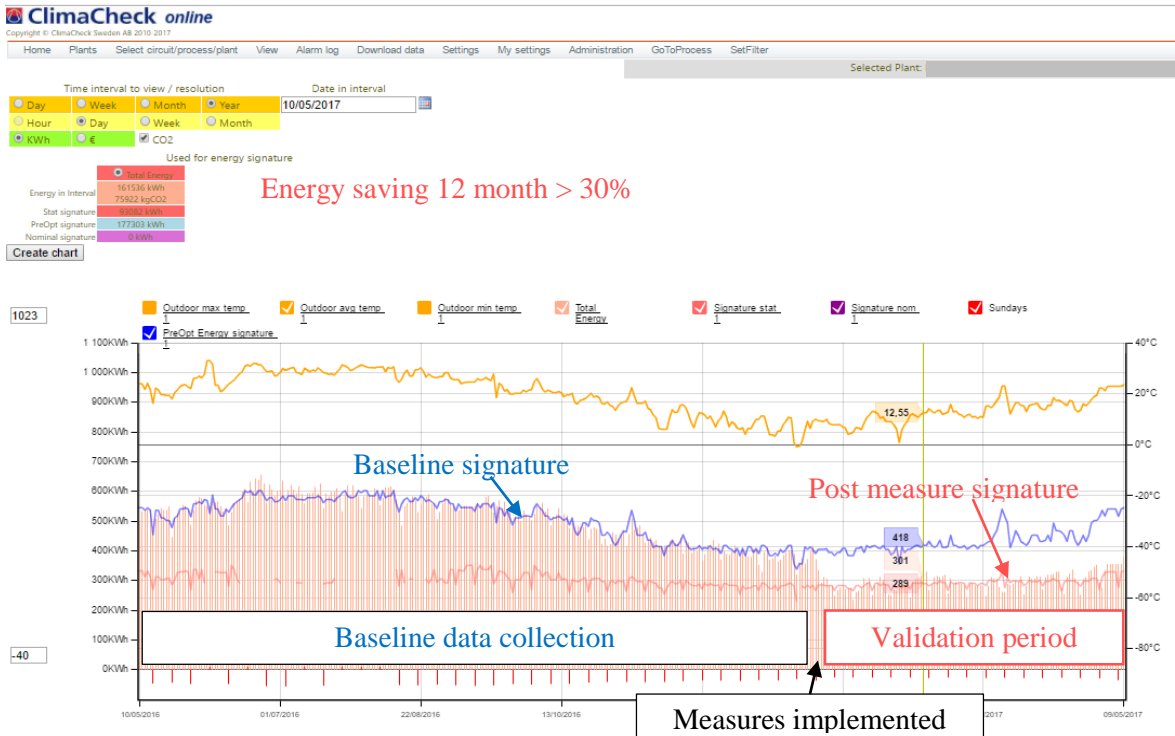
Figure 3, Energy optimisation of supermarket
