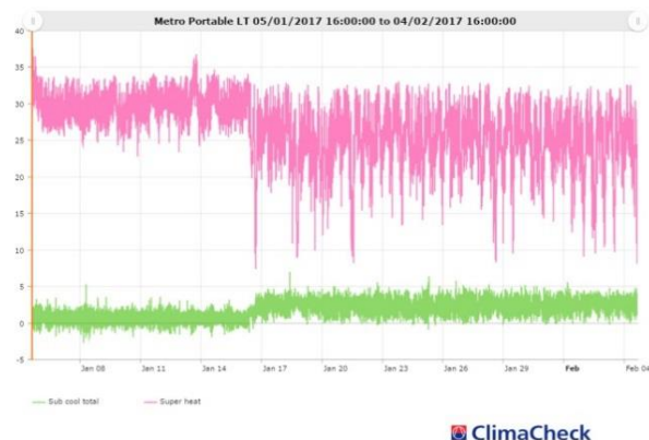
Figure 6, Subcool and Super heat before and after measures
