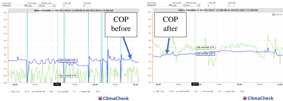
Figure 4, COP before and after measures
